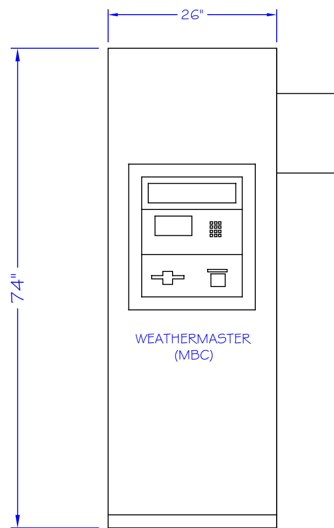
FRONT ELEVATION SCALE: 1/2" = 1'
