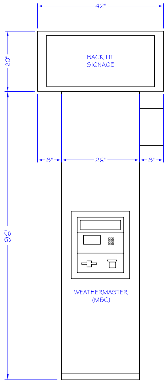
FRONT ELEVATION SCALE: 1/2" = 1'
